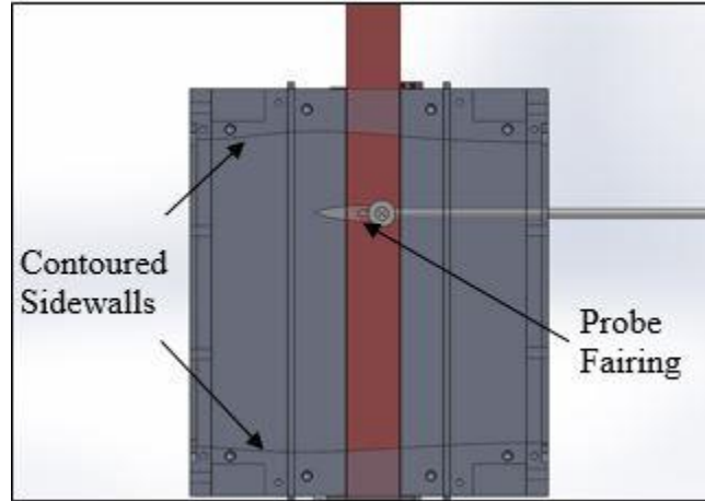
Figure 14: Cutaway of traversing section duct.
