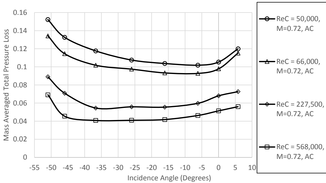
Figure 95: Mass averaged total pressure loss buckets as a function of Reynolds number and incidence angle under high turbulence.
